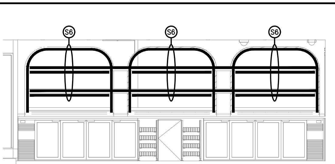
DETAIL B GAMING BAR REAR WALL ELEVATION SCALE 1: 50
