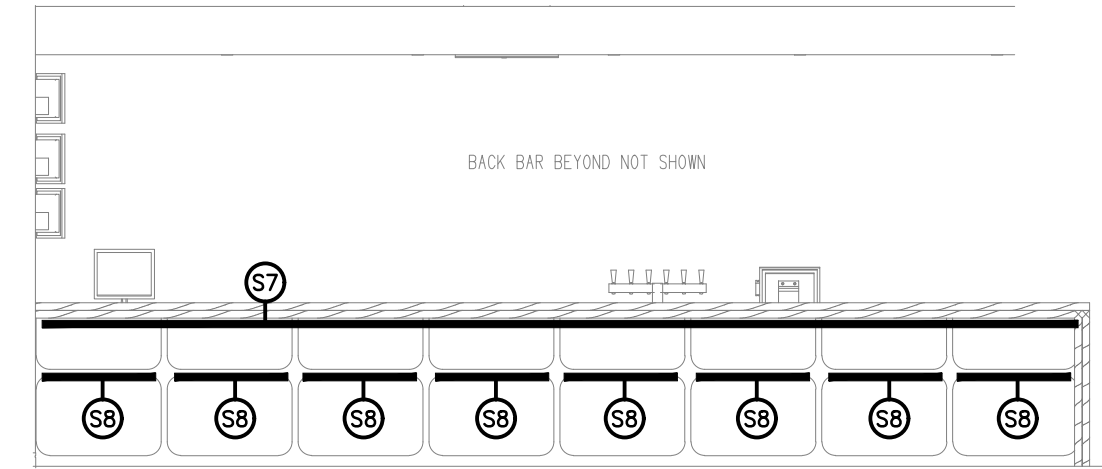
DETAIL C GAMING BAR FRONT COUNTER ELEVATION SCALE 1: 50
