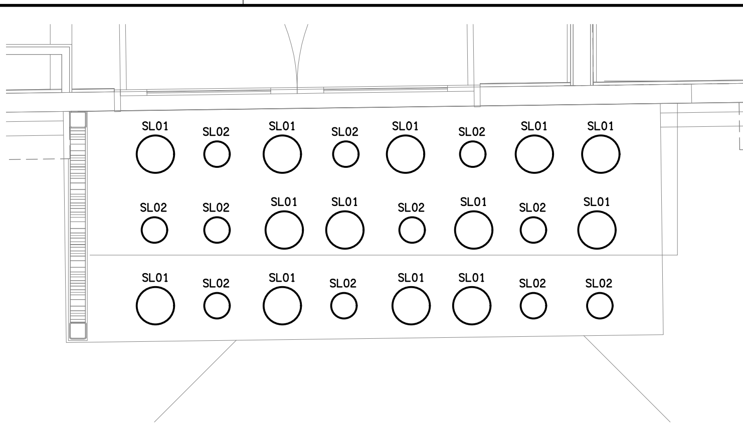
DETAIL A ENTRY FEATURE LIGHTING PLAN SCALE 1: 20
