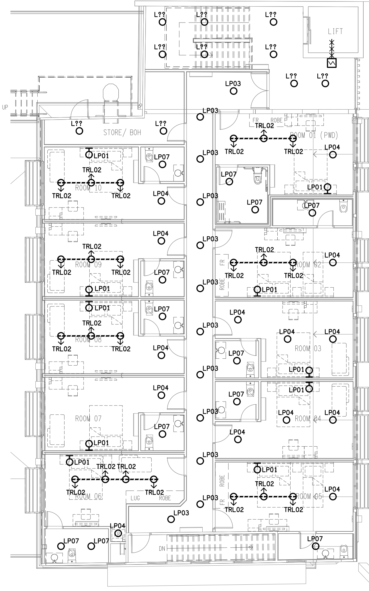
LEVEL 1 REFLECTED CEILING PLAN SCALE 1: 100
