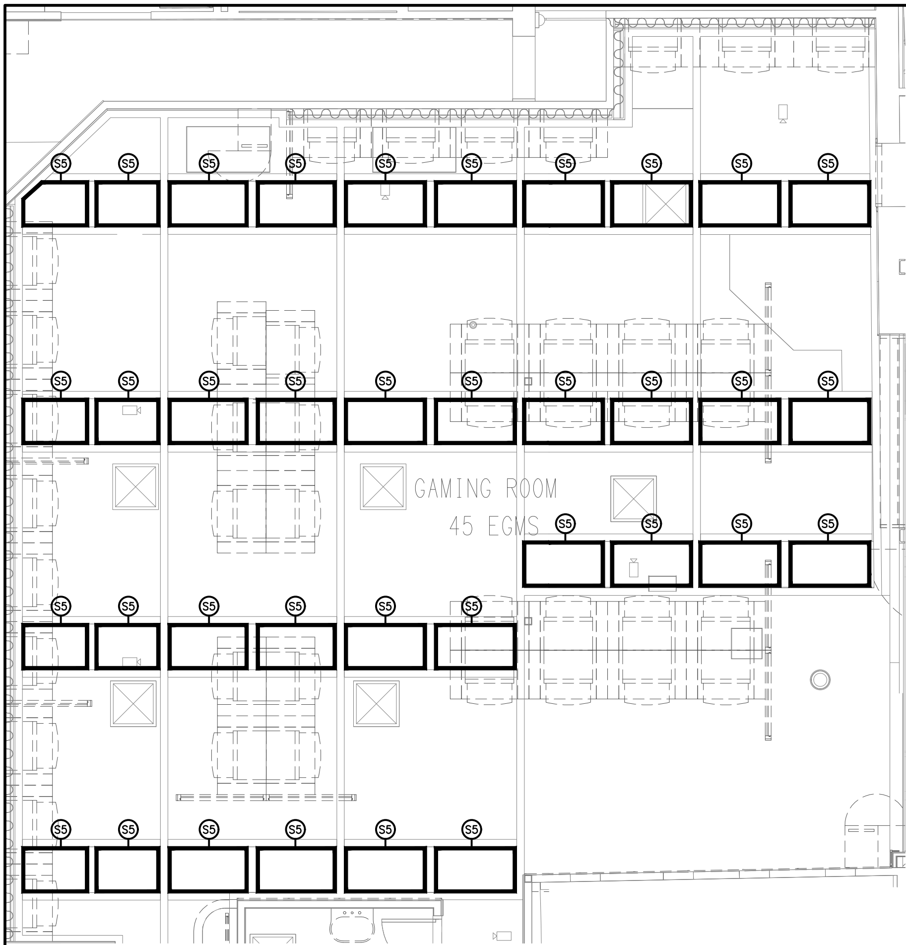
DETAIL B GAMING ROOM S5 FEATURE LIGHTING PLAN SCALE 1: 50
